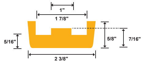
Redco™ 81X ● 3" Steel Channel Insert (For 3 x 4.1lb Steel Channel) Part #: R-28855
