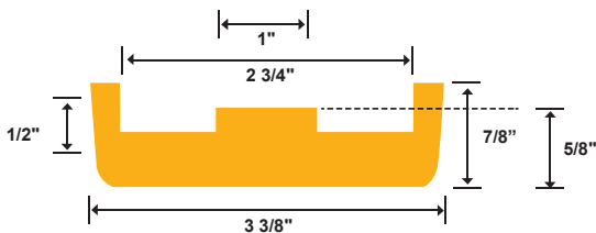
Redco™ 81XHH ● 4" Steel Channel Insert (For 4 x 5.4lb Steel Channel) Part #: R-28857
