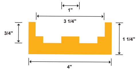
Redco™ 81XHH/C188/H78 E Trak Channel Part #: R-10148-E
