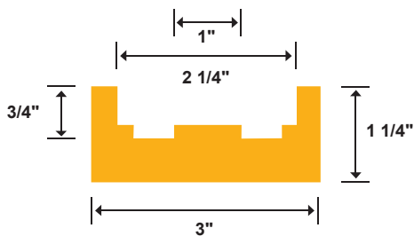
Redco™ 81X E Trak Channel ● Part #: R-5007-E
