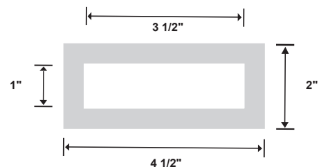
Redco™ Flyte Profile For Press Over 1 x 3 1/2 Flat Bar Part #: R-4255
