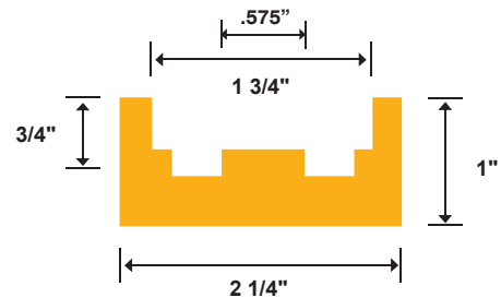
Redco™ 2080/2080H E Trak Channel Part #: R-44004-E
