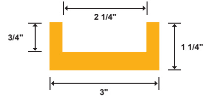
Redco™ 81X Channel ● Part #: R-5007
