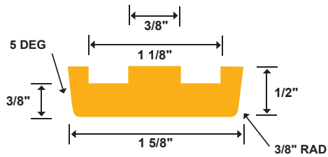
Redco™ C2060 2" Steel Channel Insert Part #: R-28853
