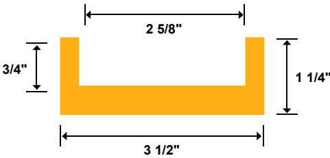
Redco™ HD-81X Channel Part #: R-10576
