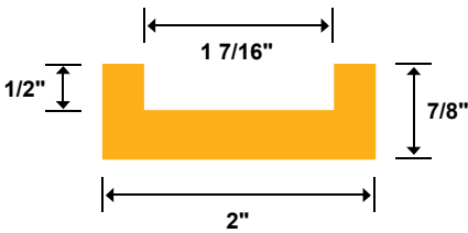
Redco™ C2060 Channel Part #: R-13858
