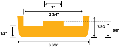
Redco™ 81XHH 4" Steel Channel Insert (For 4 x 5.4lb Steel Channel) Part #: R-28857
