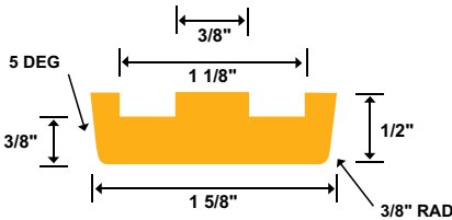
Redco™ C2060 2" Steel Channel Insert Part #: R-28853
