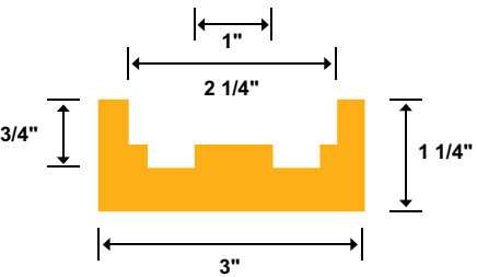
Redco™ 81X E Trak Channel Part #: R-5007-E
