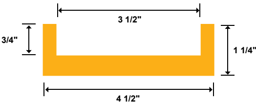
Redco™ H82 Channel H82, WR78HD, WR82 Part #: R-4540
