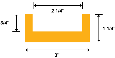
Redco™ 81X Channel Part #: R-5007
