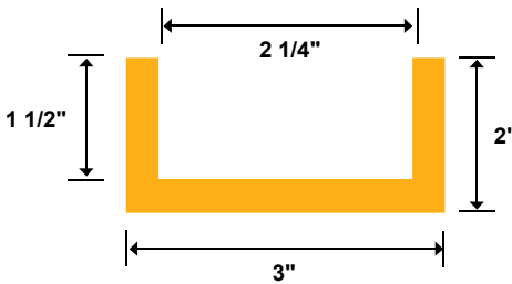
Redco™ 81X High-Side Channel Part #: R-9087
