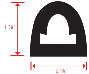
D-Shaped Fender
